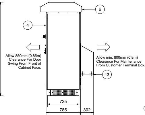
Side View (Right) AVR Cabinet Enclosure
