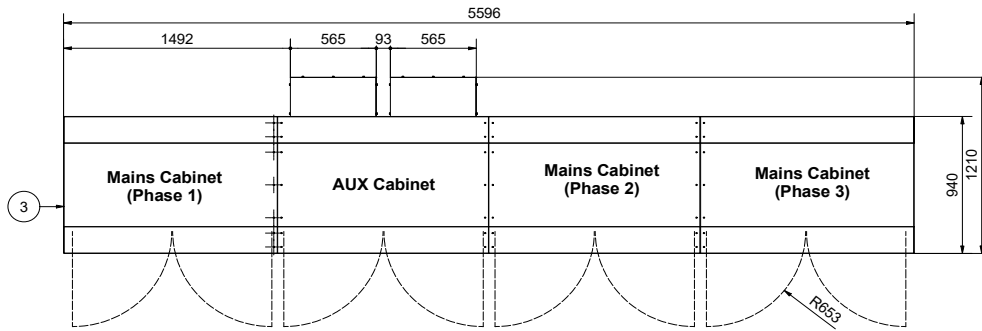
Top View - AVR Cabinet Enclosure
