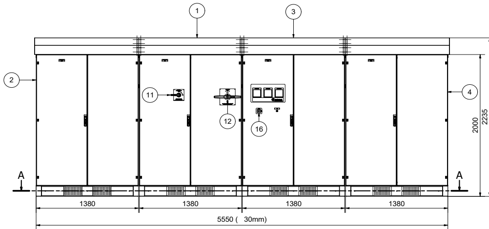
Front View - AVR Cabinet Enclosure
