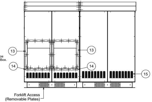
Rear View (Right) - AUX and one AVR Cabinet Enclosure
